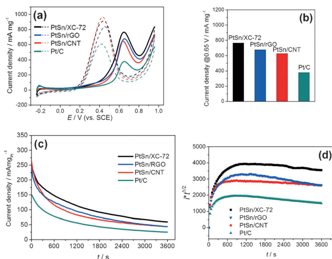
Figure 4. a) CV curves recorded from electrodes coated with synthesized PtSn/XC-72 (Figure 2), PtSn/rGO (Figure 3 d–f), PtSn/CNT (Figure 3 a–c), and commercial Pt/C in an aqueous solution of H 2 SO 4 (0.5 M) and C 2 H 5 OH (1 M) at room temperature. Scan rate (50 mV s -1 ), current densities normalized against the mass of metallic Pt loaded onto the electrodes. b) Comparison of the current density ( i ) over time ( t ) at 0.65 V (vs. SCE) for electrodes modified with different catalysts. c) Chronoamperometric curves measured at 0.45 V (vs. SCE) for electrodes modified with different catalysts. d) Calculated i t 1/2 as a function of time.
